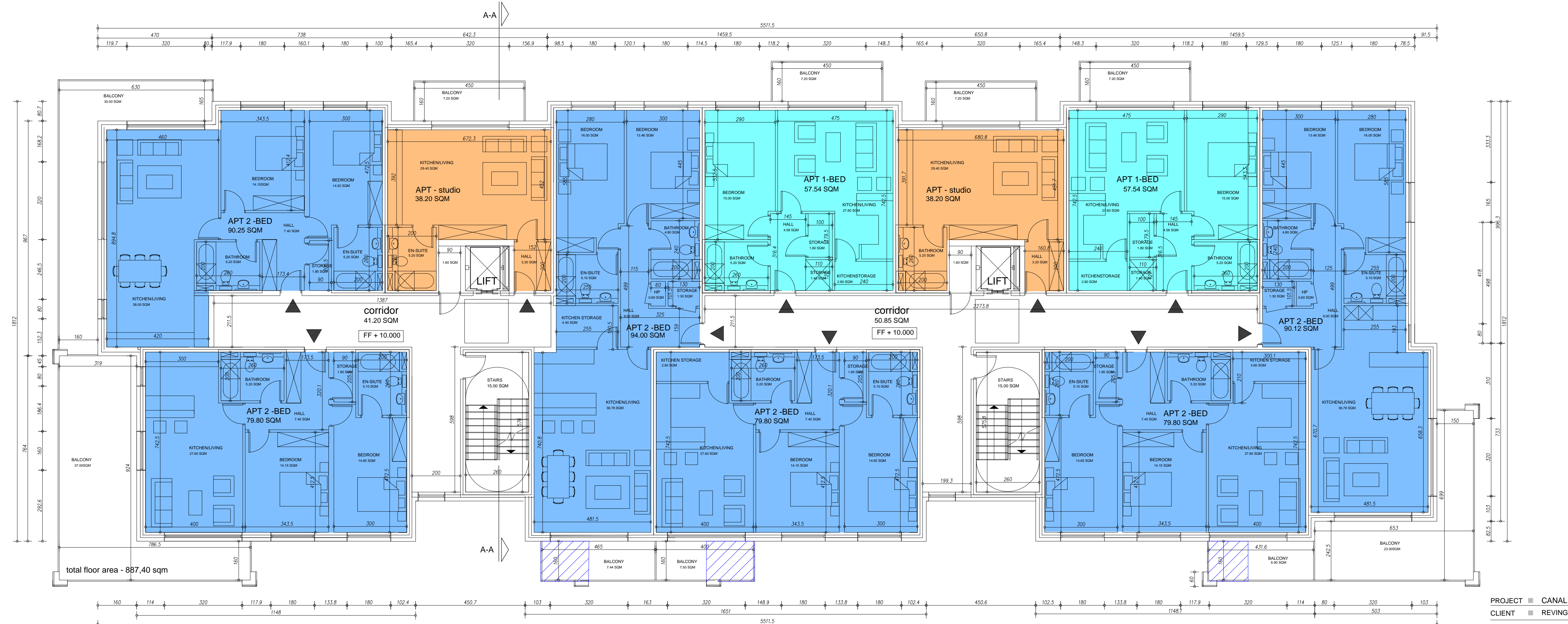
1 PROPOSED BLOCK 5 - 1st-4th FLOOR PLAN 1:100
