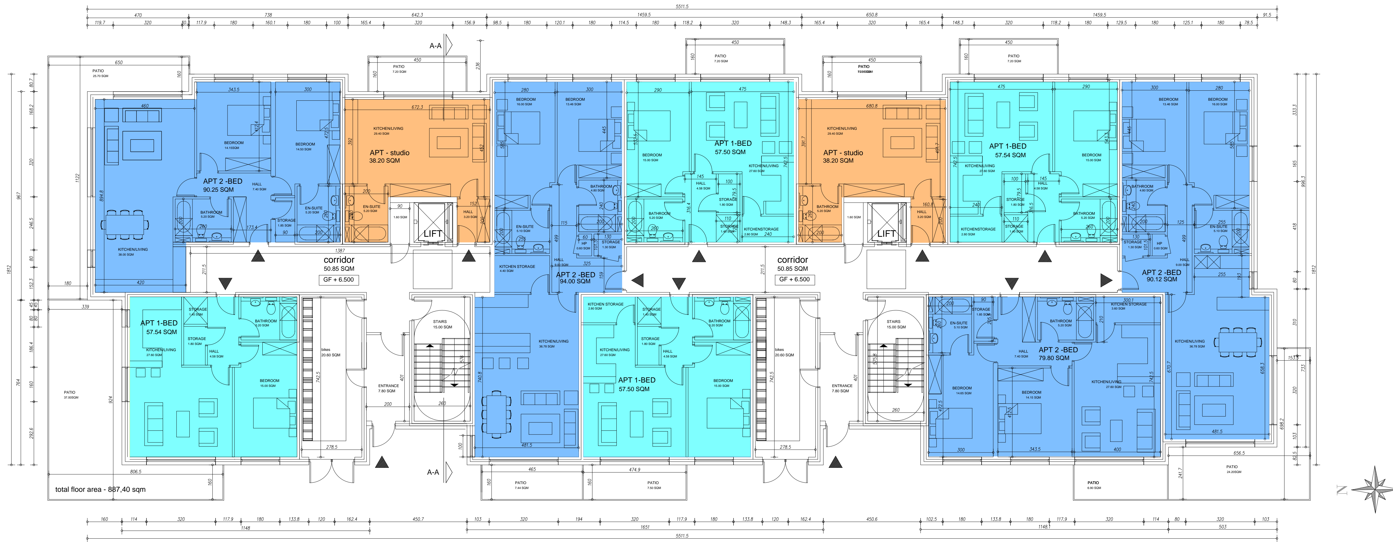
1 PROPOSED BLOCK 7 - GROUND FLOOR PLAN 1:100
